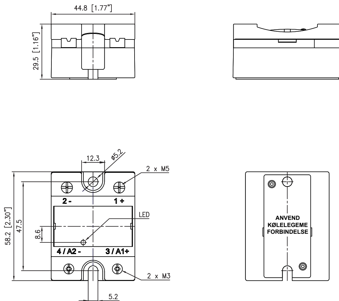
Fig. 1 RM1D dimensioner
