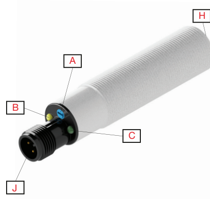
Fig. 2 CA18 Conector
