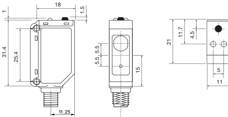
Fig. 10 Conector
