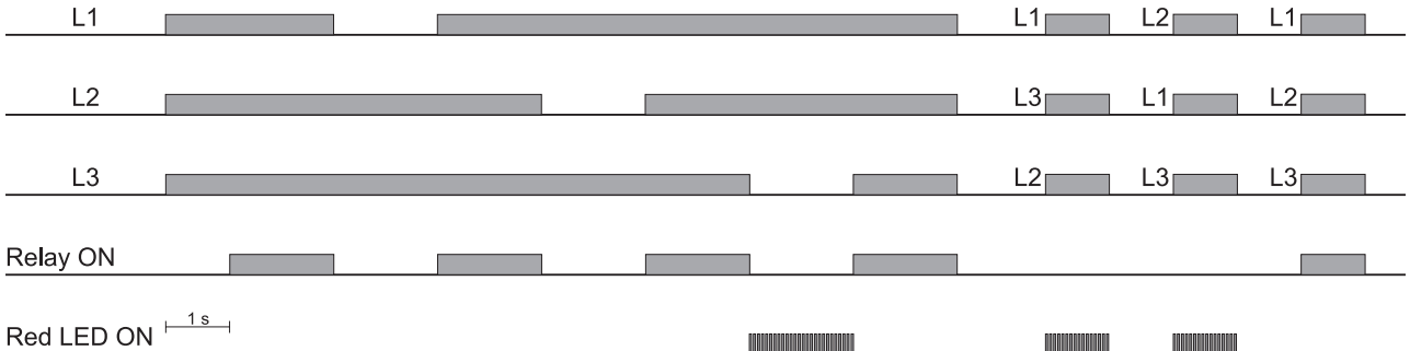
Fig. 2 Phase sequence, total phase loss
