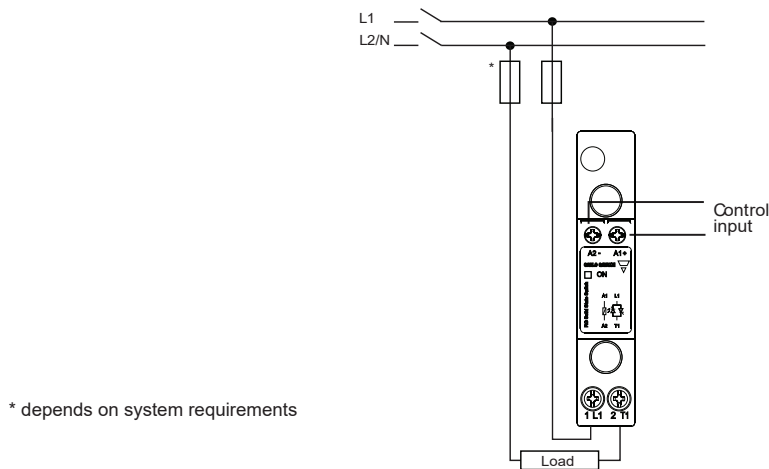
AC control
